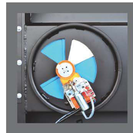
Combustion air control closed
